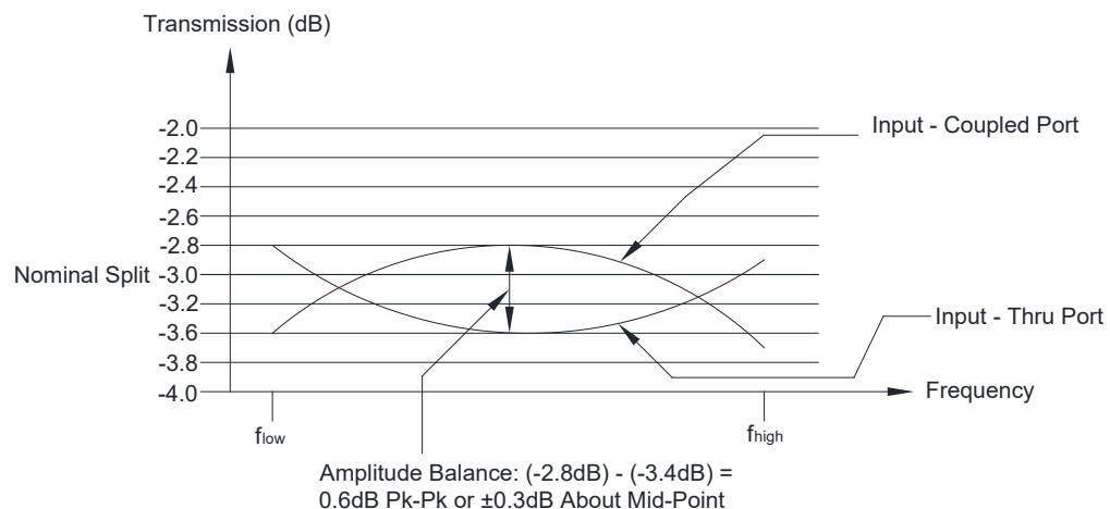
Typical Amplitude Balance Response for 1-Section Coupler
