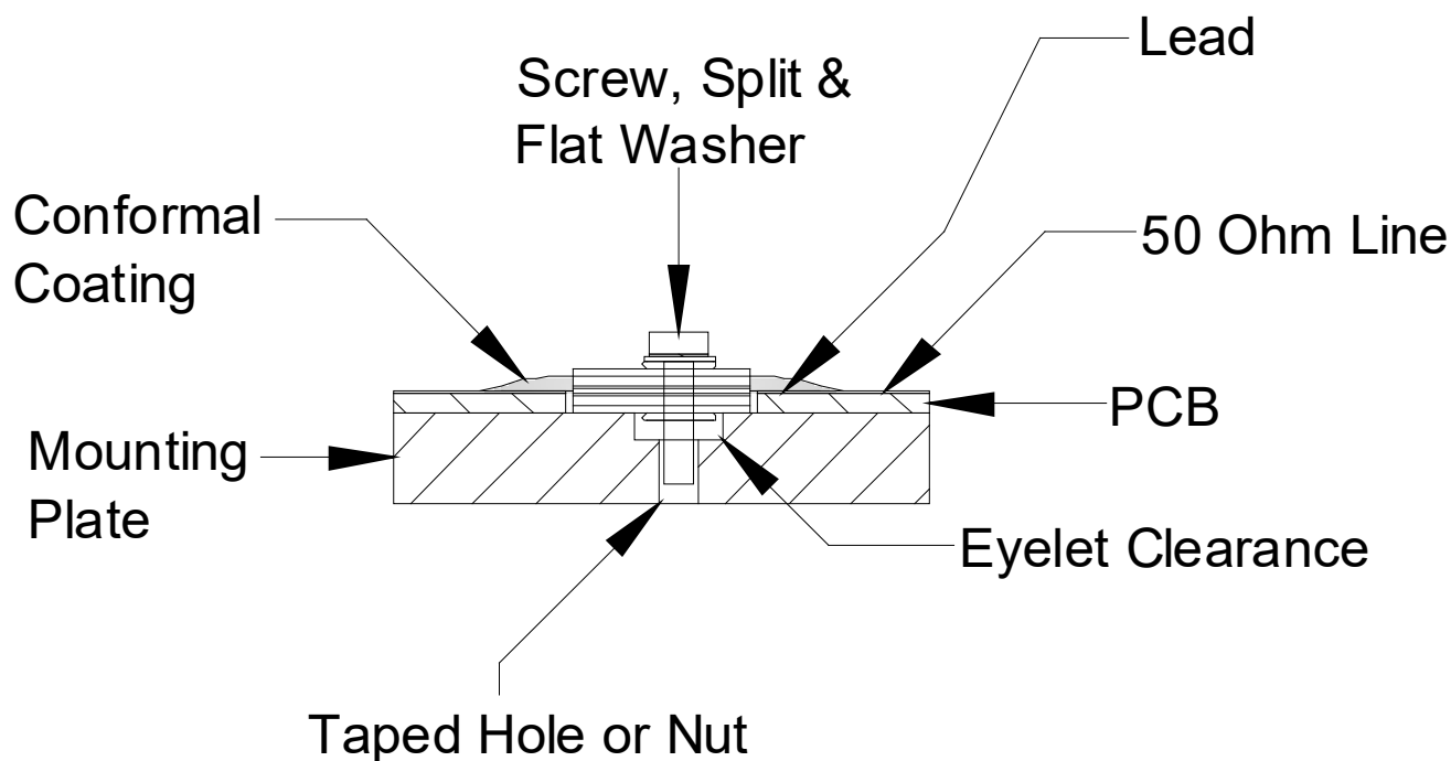
Mounting, Side View
