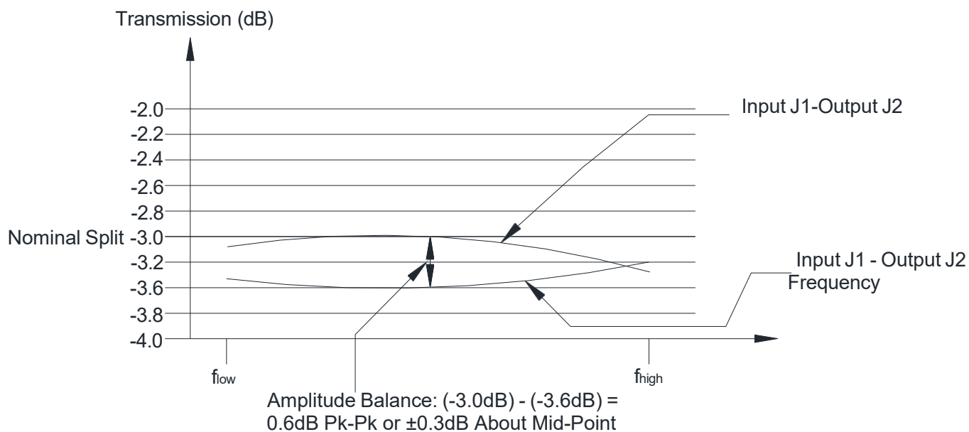
Typical Amplitude Balance Response
