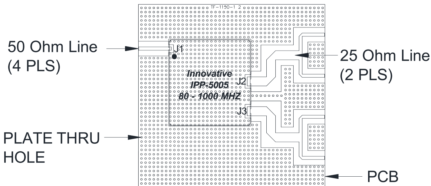
IPP Balun Test Fixture
